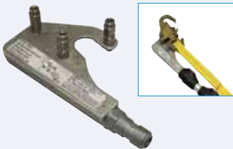
Remote Saphook Connector 3021-1 Attaches to end of 3022-1 pole and allows user to attach 3006 saphook to overhead anchorage point. May also be used for a remote connection in rescue scenarios.
