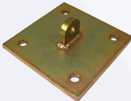
Rebar Anchor Lug Plate for Concrete Construction 3083-12
