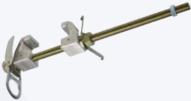
Adjustable Beam Anchor 3093-1 Fits I-Beams with 4" -16-5/8" flanges & 1/4" - 1-3/4" flange thickness
