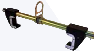
Adjustable Sliding Beam Anchor 3097-1 Fits flange 5-1/2" - 18" wide & 1/4" - 2-1/2" thick
